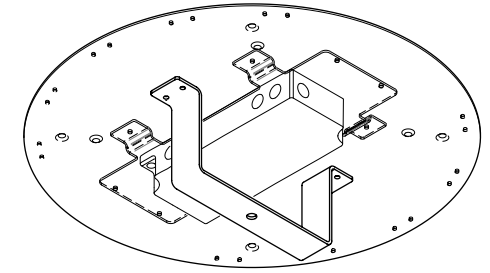
Canopy Assembly
